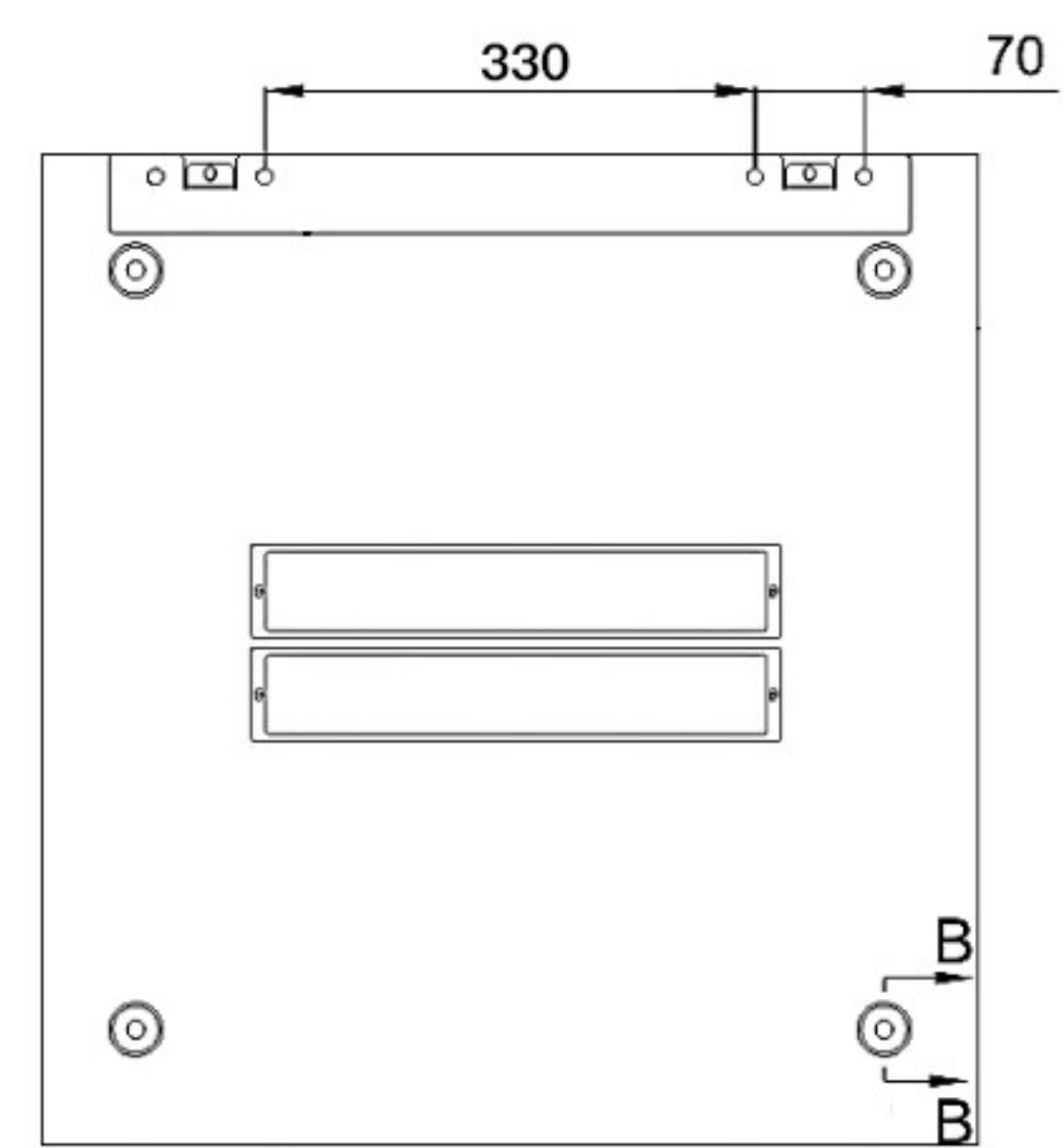
Back(wall-mounted hole size)
