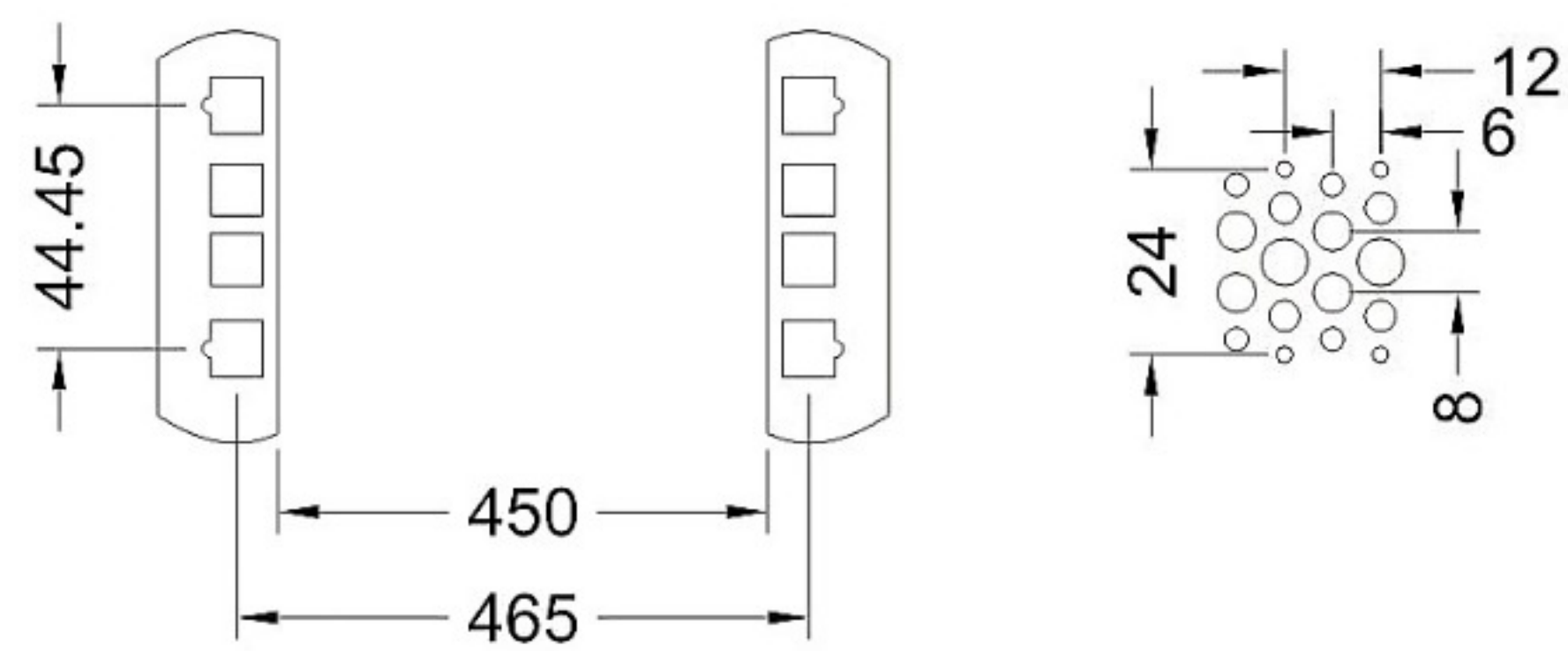
Mounting dimension
